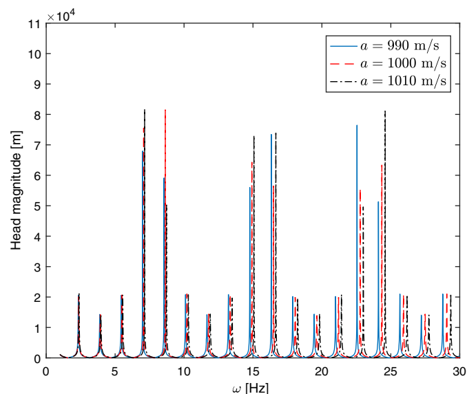
Fig. 11. Head response at x^M = 2,000 m in the frequency domain with unit input discharge perturbation at the valve with different wave speed a = 990, 1,000 , and 1,010 m/s. The leak location is at x^L = 400 m.
